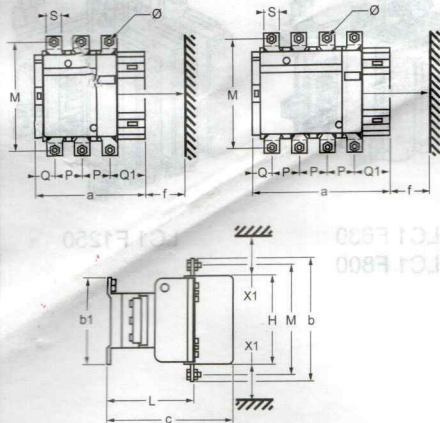
LC1 F115...F330
