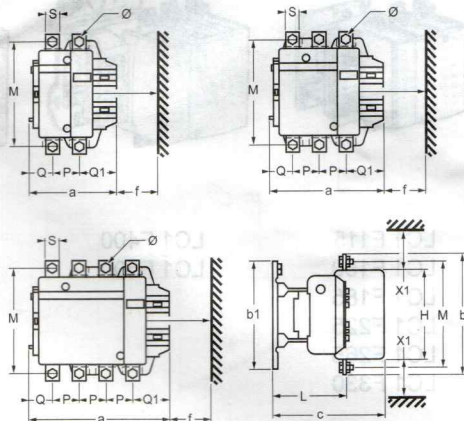
LC1 F400...F500
