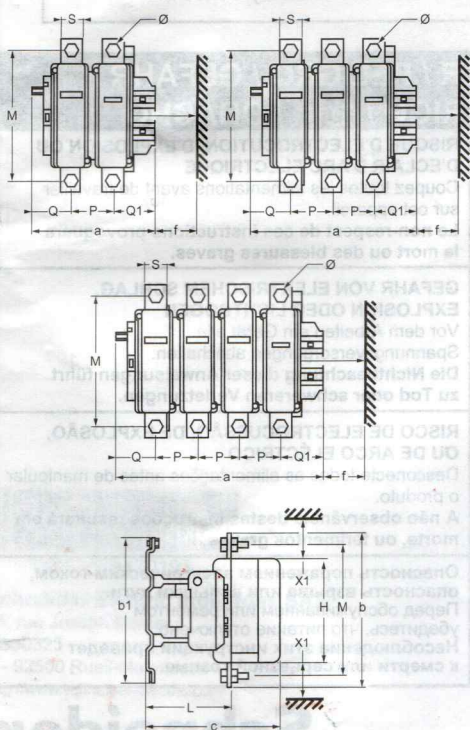
LC1 F630...F800
