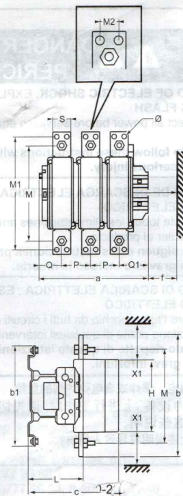
LC1 F1250
